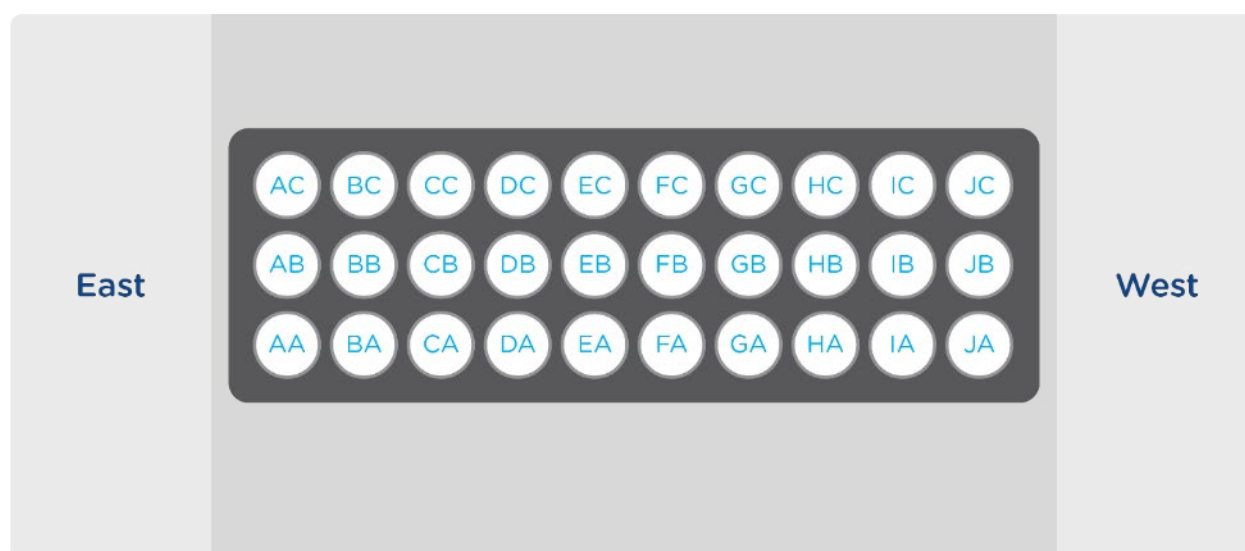
Figure 7: Duct naming convention
