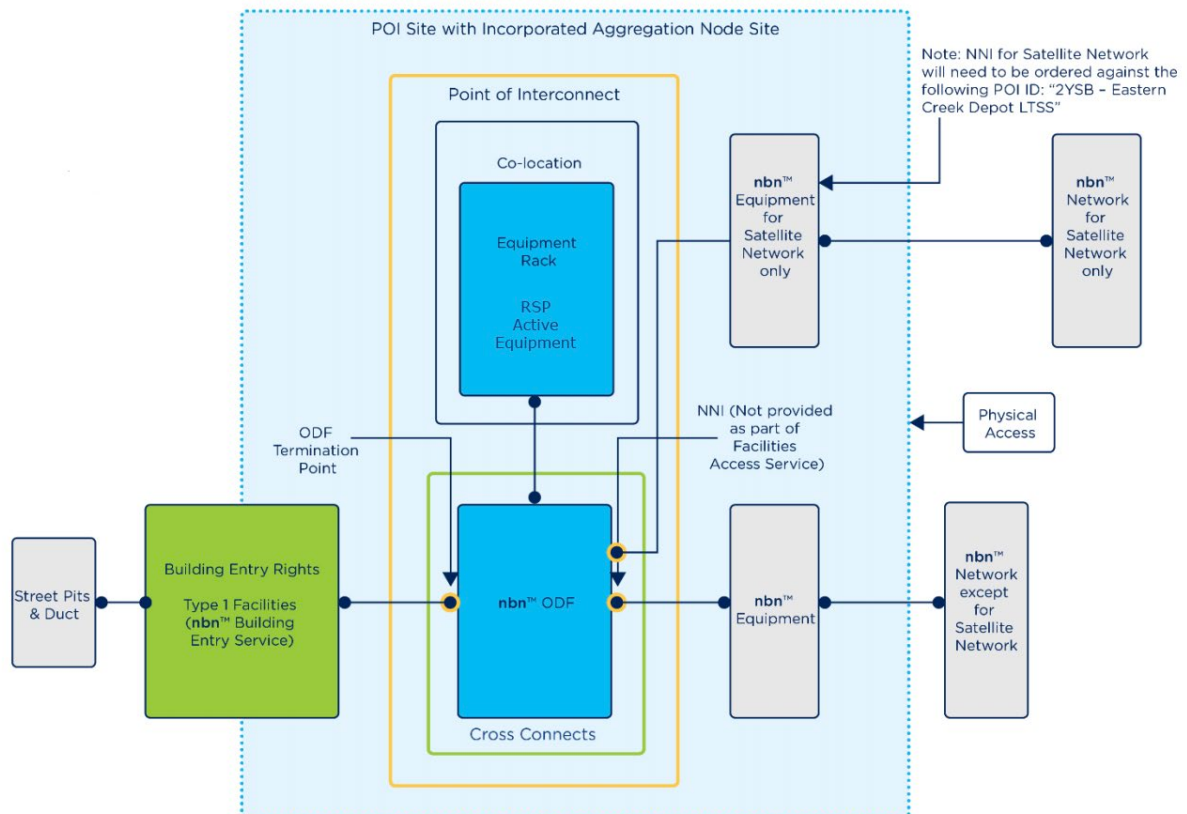
Figure 3: Relationship between different Service Elements of the Facilities Access Service at the Eastern Creek POI Site
