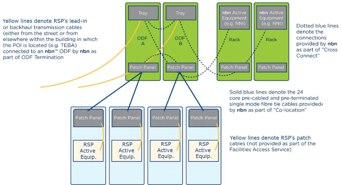
Figure 4: Type of interconnection that can be achieved using a combination of ODF Termination, Cross Connect and Co-location
