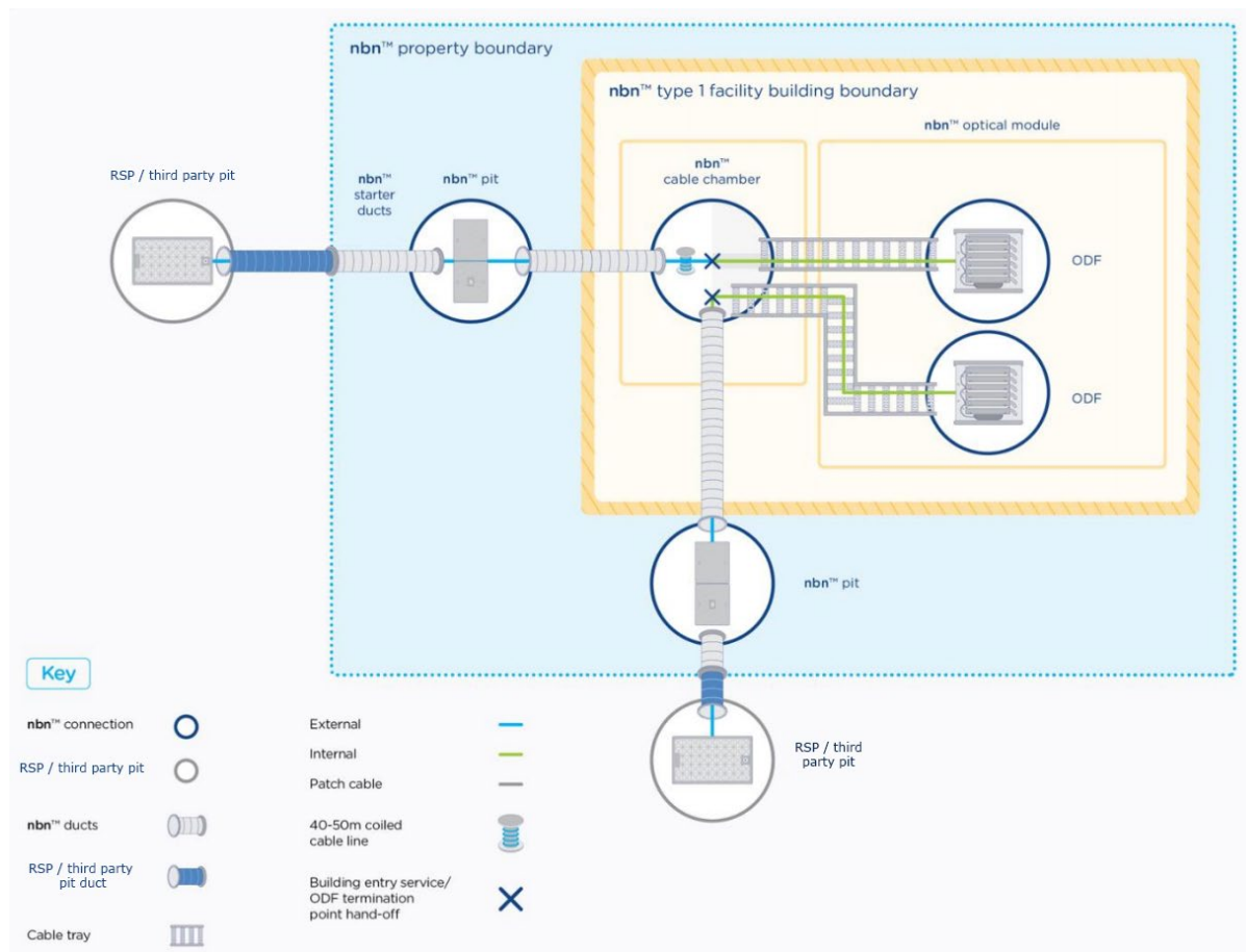
Figure 8: nbn® Building Entry Service highlighting diverse fibre entry
